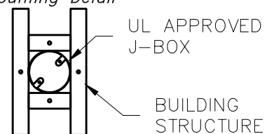
Mounting Detail
