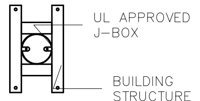
Mounting Detail
