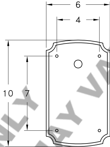
MOUNTING DETAIL
