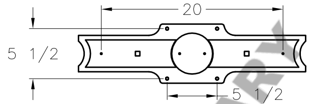
MOUNTING DETAIL
