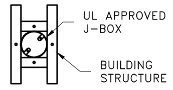
Mounting Detail
