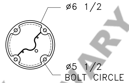
MOUNTING DETAIL
