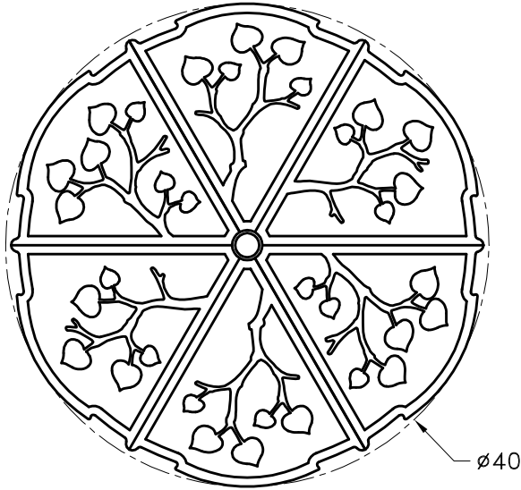
BOTTOM VIEW (NOT TO SCALE)
