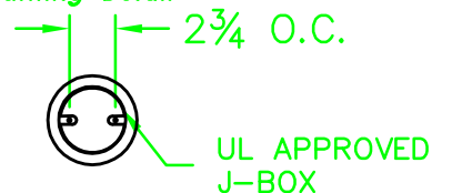
Mounting Detail
