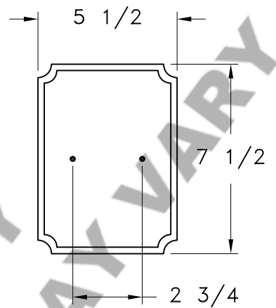
MOUNTING DETAIL
