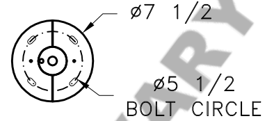
CANOPY DETAIL
