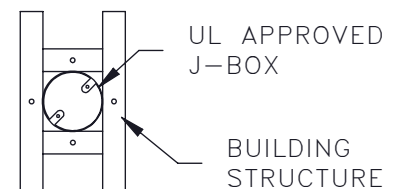
Mounting Detail
