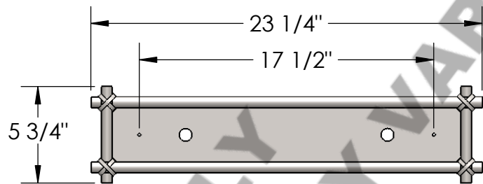
MOUNTING PLATE
